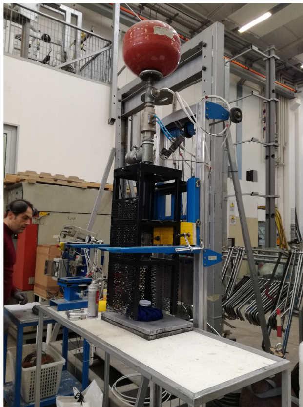
Photograph of a specimen during the test
